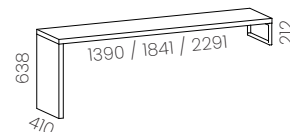
MTV3 - NK / MTV4 - NK / MTV5 - NK (L, D)
